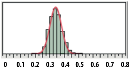
Figure 1. Idq_total, Nominal = 340mA
